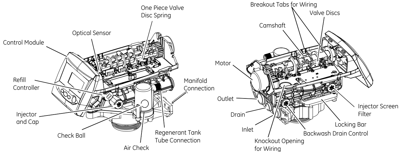
Figure 1 255 Valve Layout
