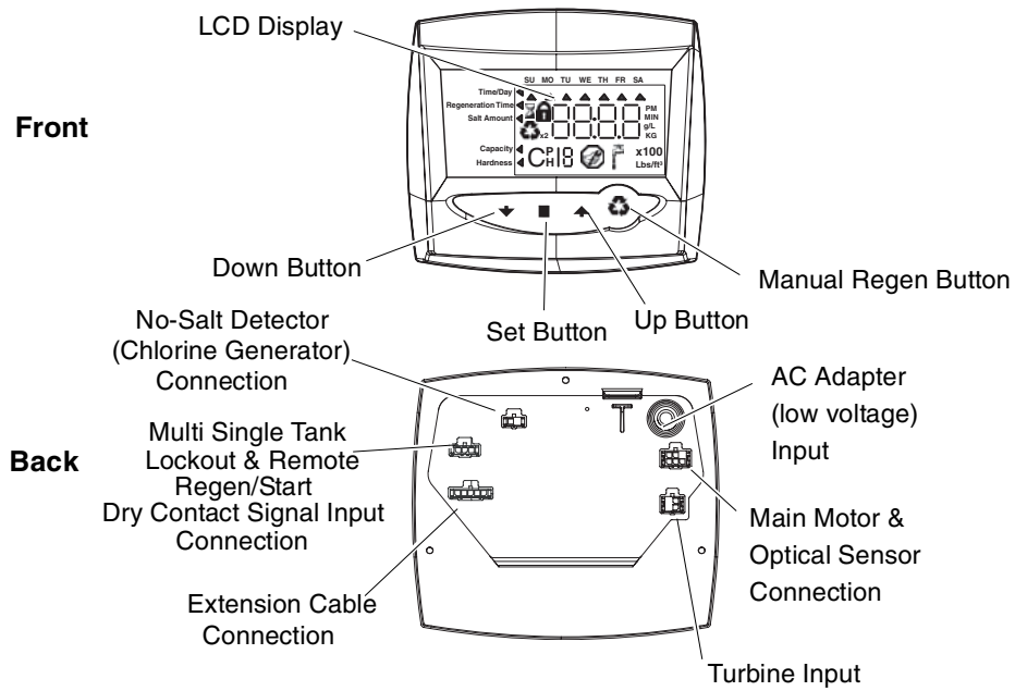
Figure 2 764 Controller Identification
